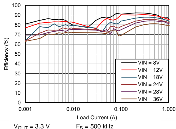
Figure 54. Efficiency
