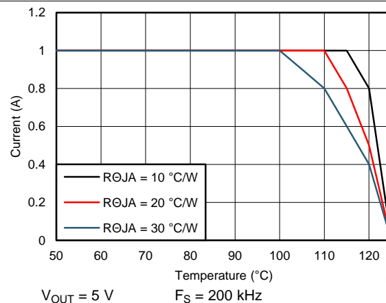
Figure 70. Derating Curve
