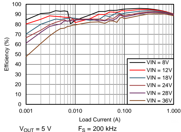
Figure 66. Efficiency
